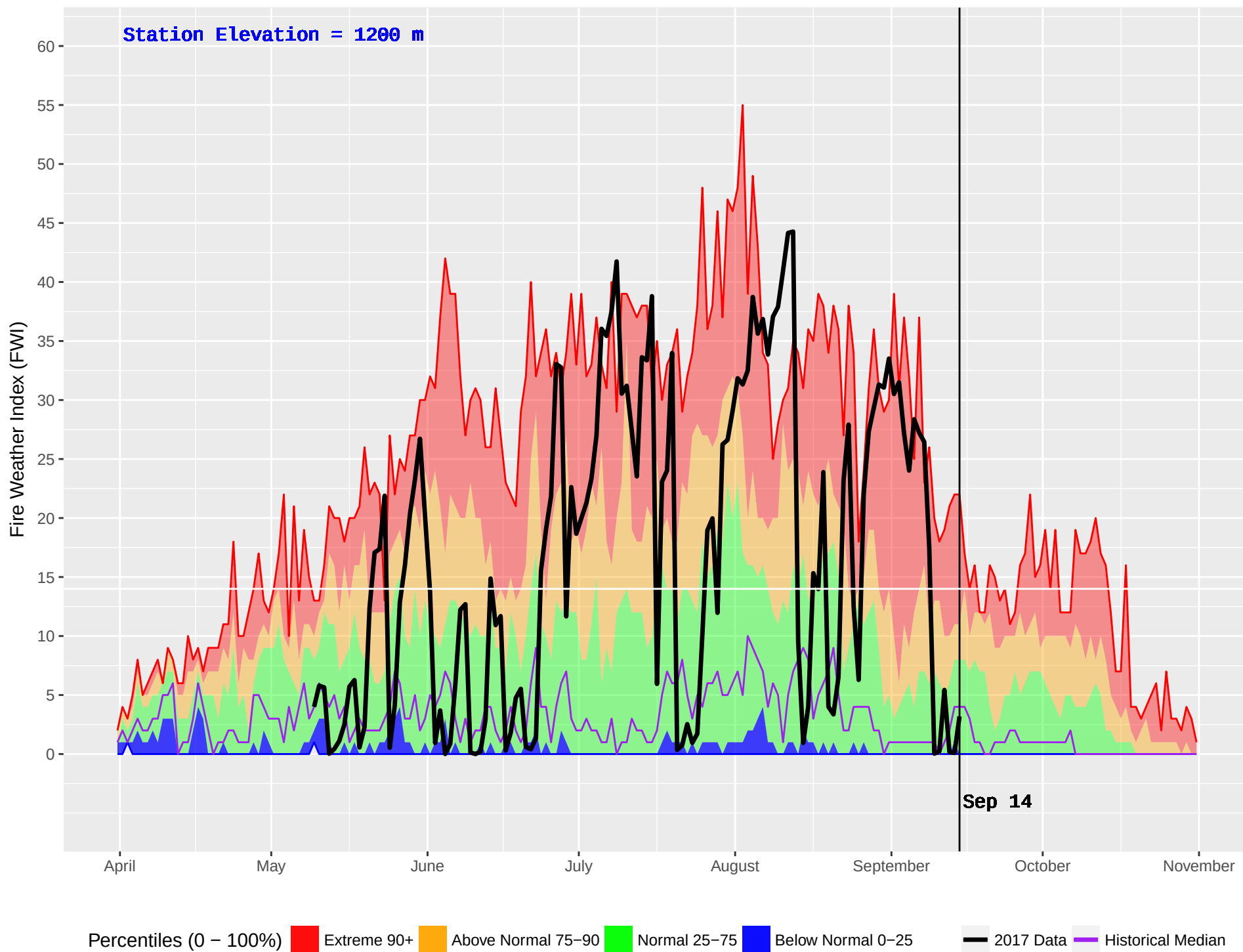
TSAR CREEK (361) : Historical (1986–2016) and Current (2017) Noon Fire Weather Index (FWI)
