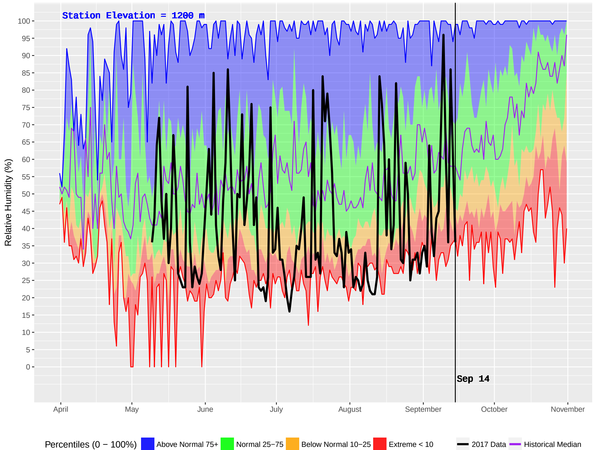
TSAR CREEK (361) : Historical (1986–2016) and Current (2017) Noon Relative Humidity
